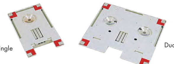
Slide Mount (suction cups & gel tape) Bottom View
