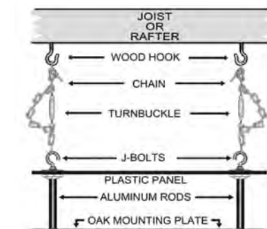
Over-the-Counter Display Tile Mounting
